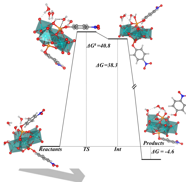
Figure 6. Reaction scheme for pNPP hydrolysis [\text{Mo}_5\text{O}_{15}(\text{pNPP})_2(\text{H}_2\text{O})_6]^{6-} . Gibbs free energies in kcal mol -1 .
