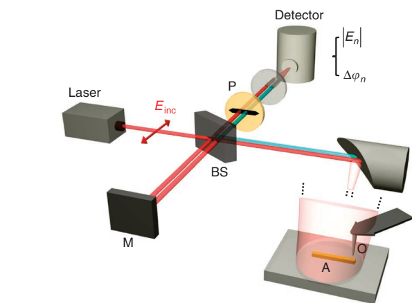
Figure 2 | Set-up for verifying surface-enhanced elastic light scattering.
